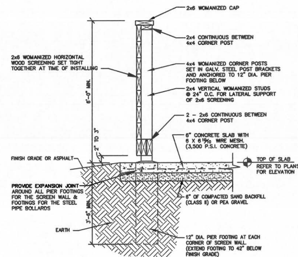
TYPICAL DUMPSTER WALL SECTION NO SCALE
