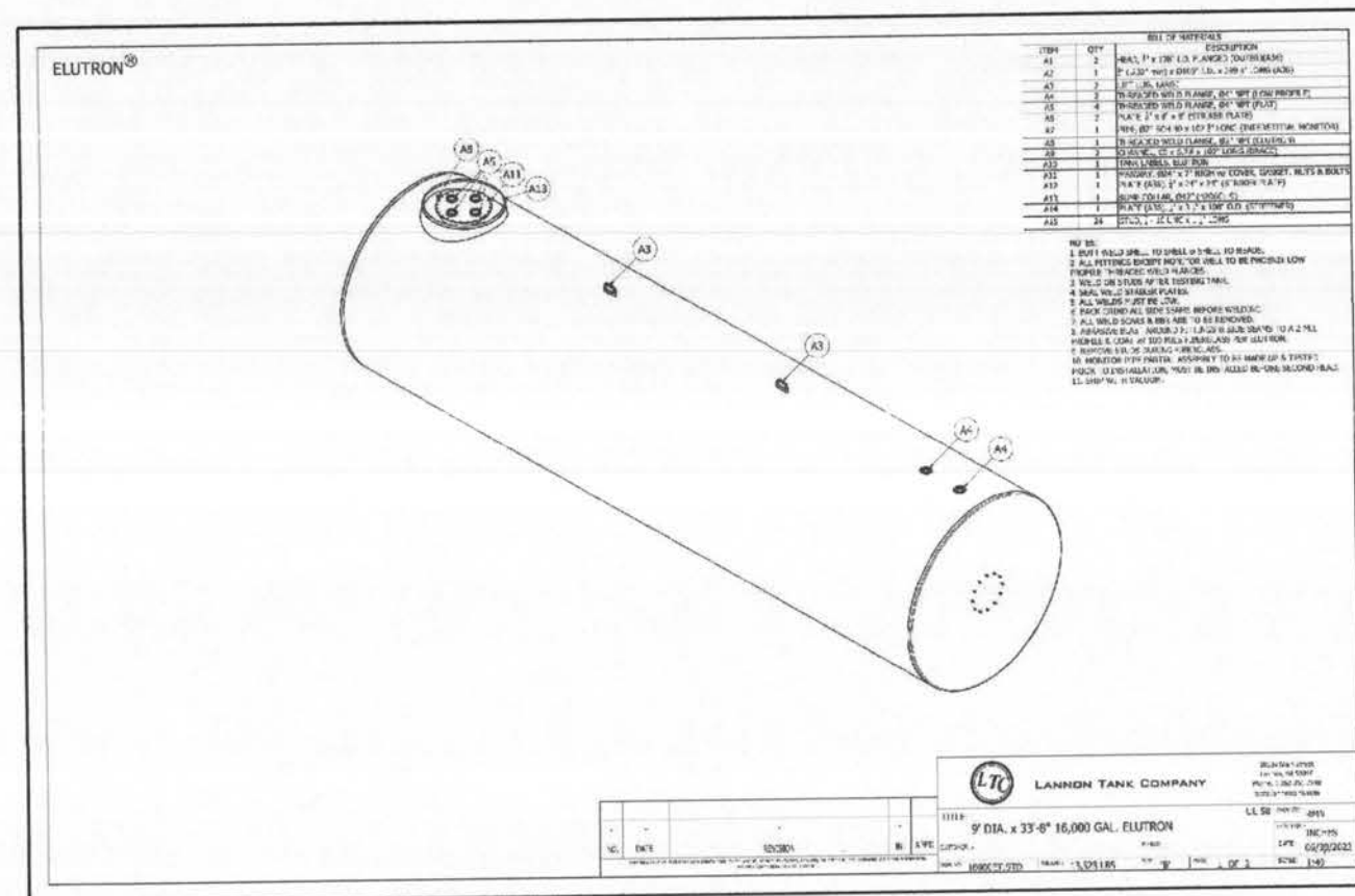
PROPOSED UNDERGROUND GAS TANKS
