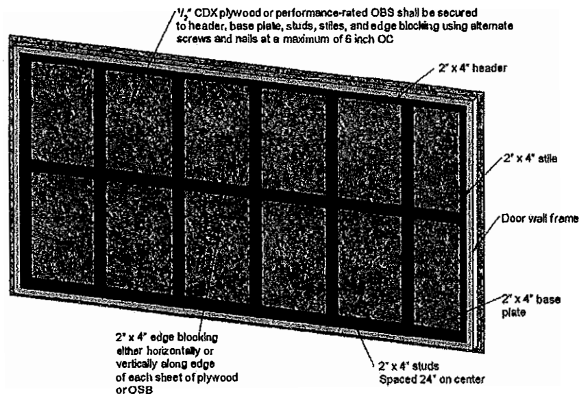
FIGURE A103.1(2) BOARDING OF DOOR WALL
